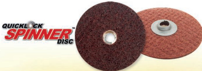
QUICKLOCK "SPINNER" 4 1/2" & 5" DIAMETER (TYPE S UNDERSIDE MOUNT WITH 5/8"-11 SCREW-ON LOCKING STYLE)
